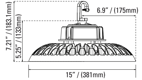
15" - 200 Watt 8.53-lbs
