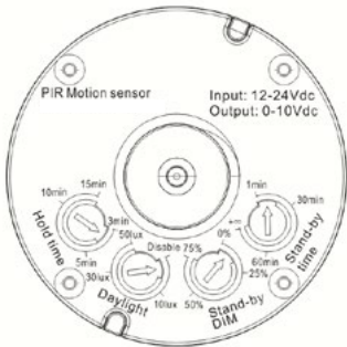
QCMS35 Accessory - Dial settings
