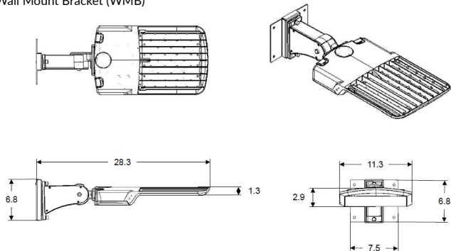
VAS Wall Mount Bracket (WMB)
