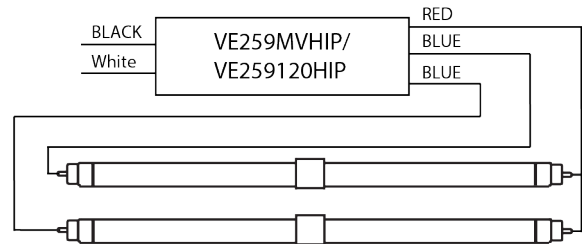
1-LAMP 120-277Vac Direct Wiring (Type B mode)
