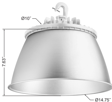
RSHL-ALR-A = 16" Aluminum Reflector for 100W/150W configurations (Sold Separately)
