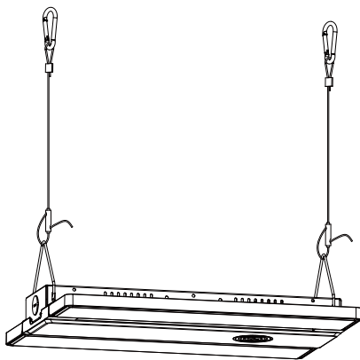
Suspension Mount
