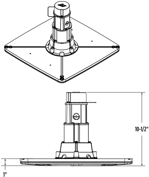
REDiMount Canopy Stiffener
