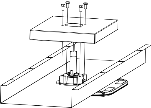
Standard Mount Canopy Stiffener
