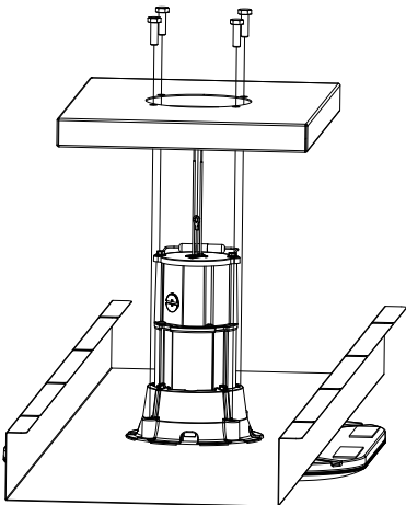
REDiMount Canopy Stiffener
