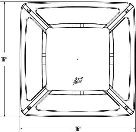
Standard Mount Canopy Stiffener
