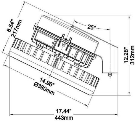
25° Stanchion mount
