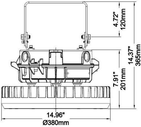
Trunnion mount
