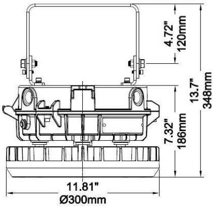
Trunnion mount
