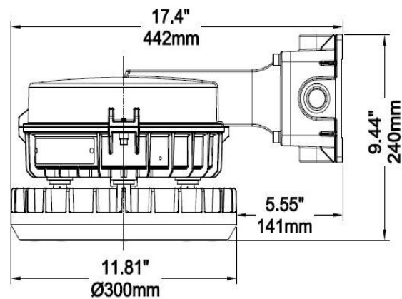
Wall bracket
