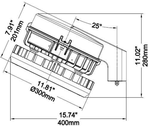
25° Stanchion mount
