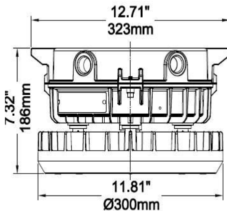
Ceiling mount
