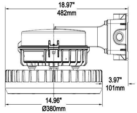
Wall bracket
