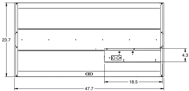
Back
