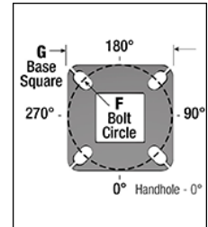
Anchorage Base Plate
