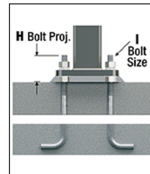
Anchor Bolts Projection & Size
